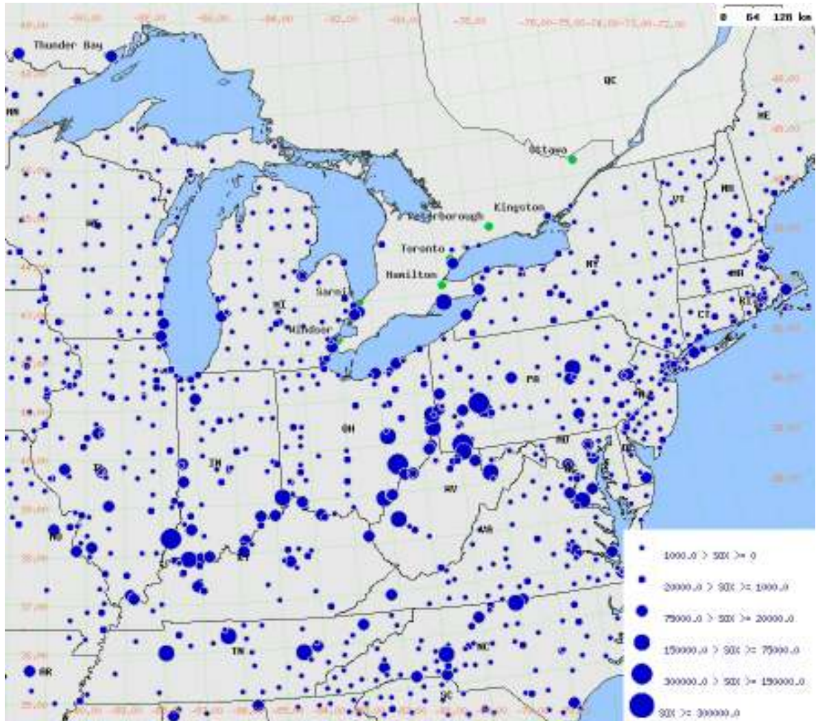
Figure A-4: Sulphur dioxide emissions from power plants shown as dots that vary in size according to their emission inventories U.S. 1995 (with 2001 updates) and Canada 1999 Emission Inventories (source: Ontario Ministry of the Environment)
