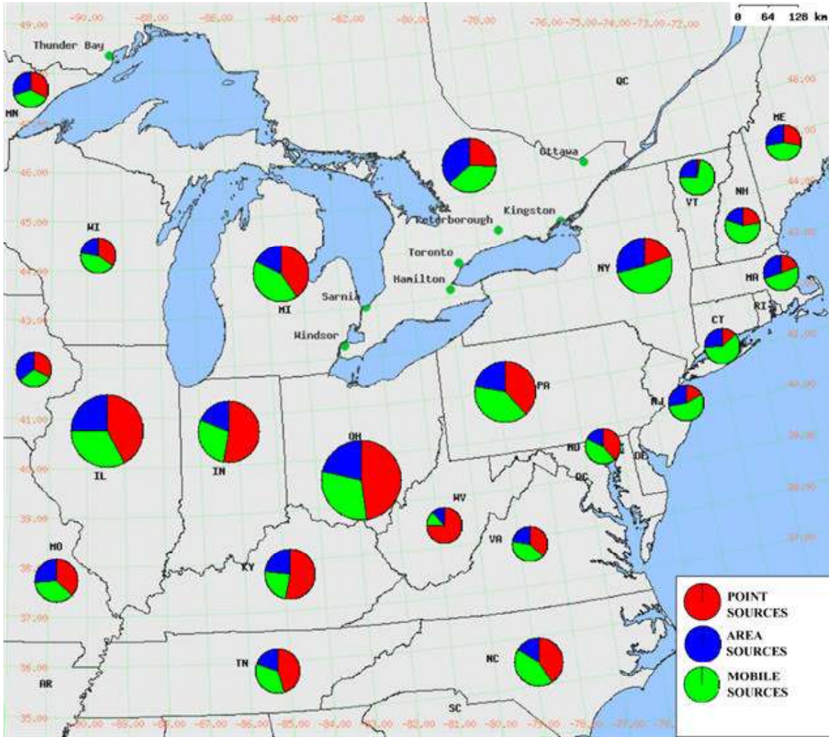
Figure 2.4: \text{NO}_x emission by source type at selected states/province. U.S. 1999 and Canada 2000 emission inventories. Pie diameter is proportional to emission scale. (source: Ontario Ministry of the Environment)
