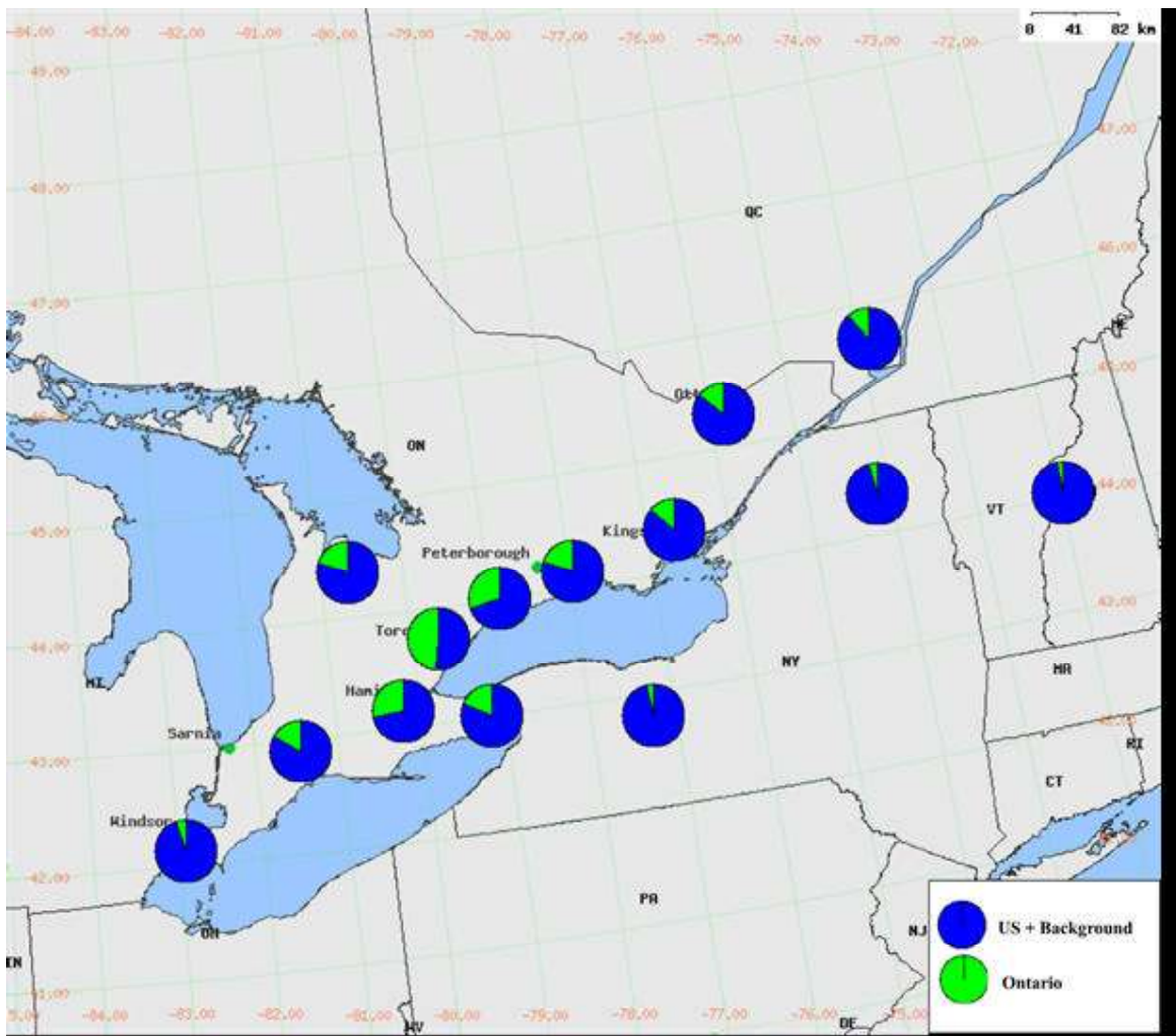
Figure 3.5: Graphic of Transboundary vs. Ontario Contribution for PM 2.5 on High Concentration Days during 1998 Spring/Summer Season. (source: Ontario Ministry of the Environment)
