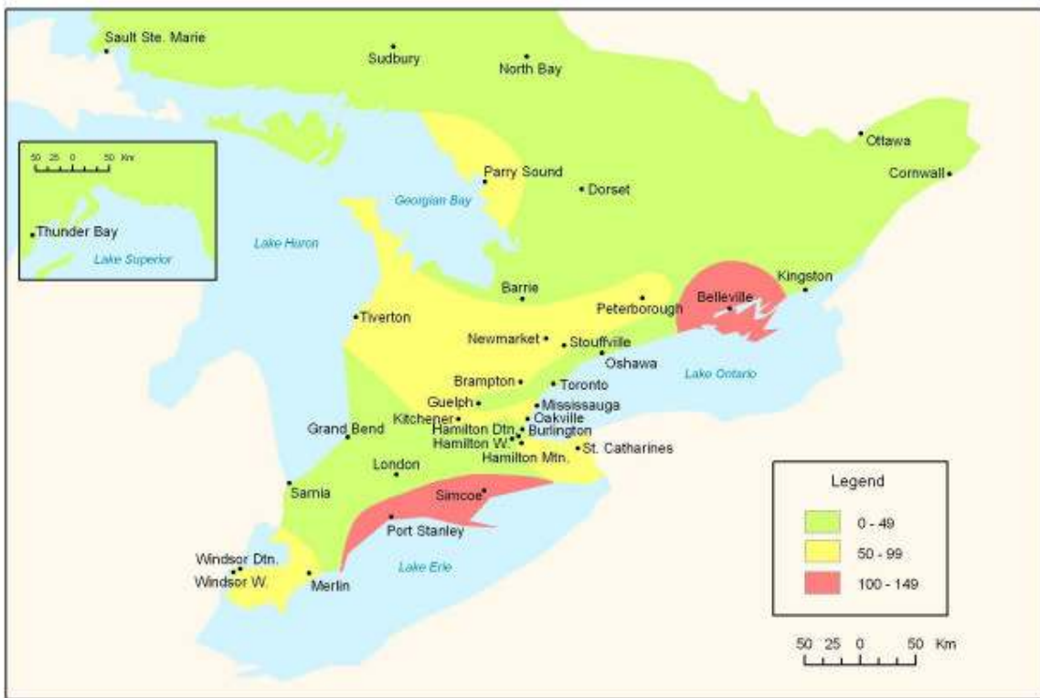
Figure 2.8: Geographical Distribution of Number of One-Hour Ozone Exceedances Across Ontario (2003) (source: Ontario Ministry of the Environment)
