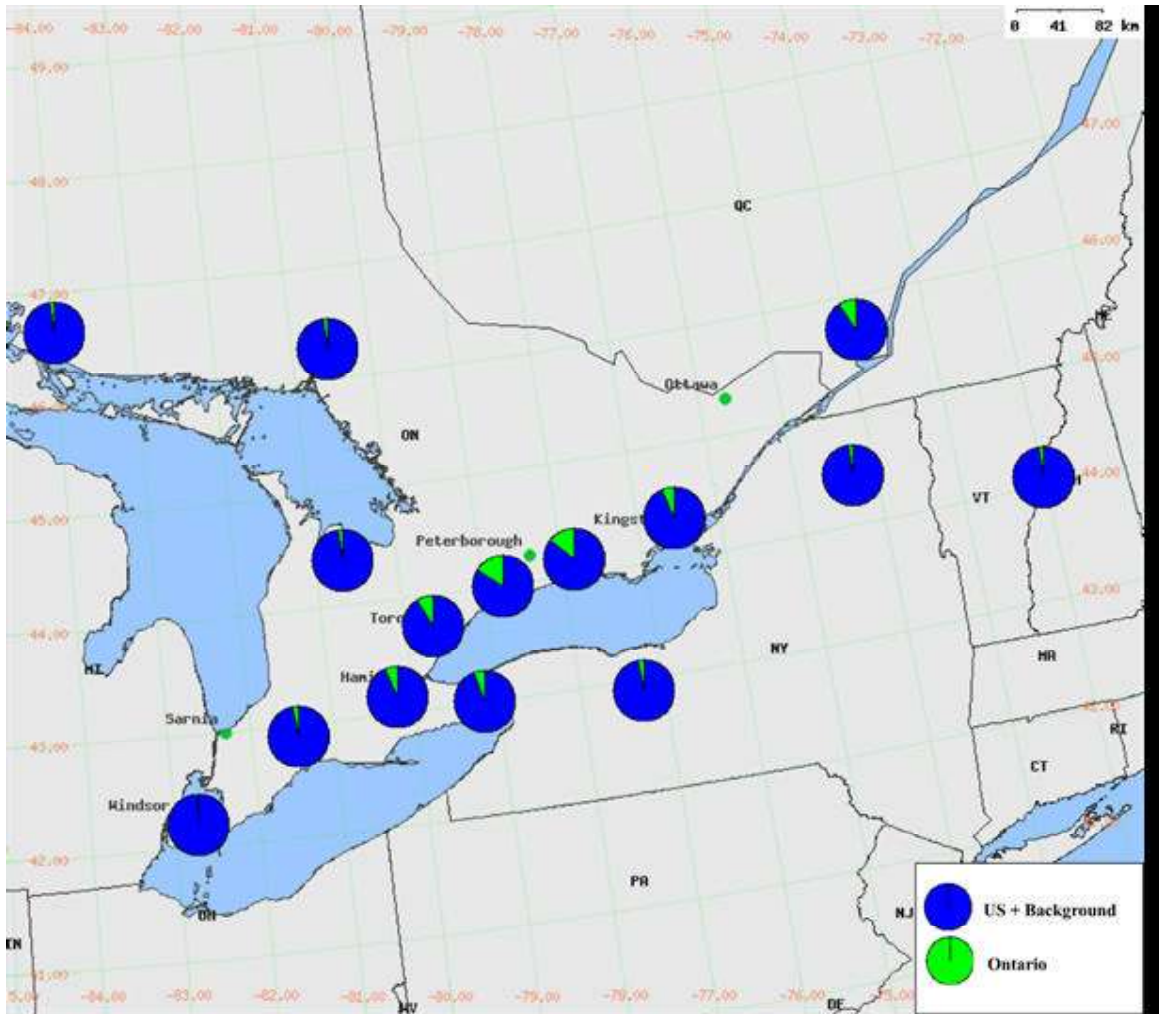
Figure 3.4: Graphic of Transboundary vs. Ontario Contribution for Ozone on High Concentration Days during 1998 Spring/Summer Season. (source: Ontario Ministry of the Environment)
